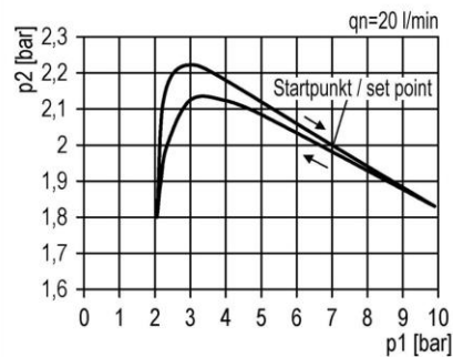
pressure characteristic
